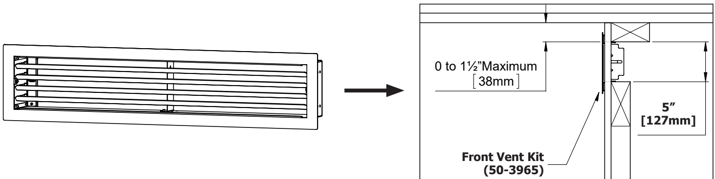
Figure 2: Front Vent Kit
